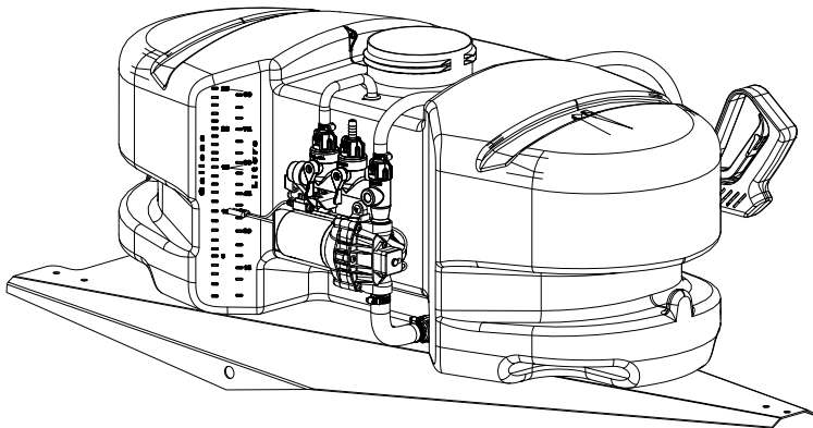
Tank/Frame Pre-Assembly
