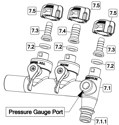
Manifold Detail See Previous Page for part numbers
