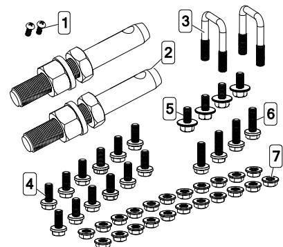
Bolt Bag (5280968)
