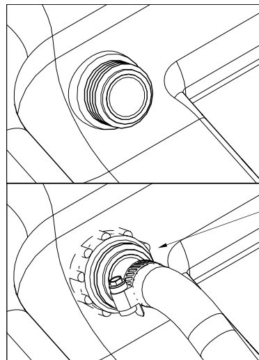
Molded-In' Inlet Fitting & Intake Sub-Assembly Attachment
